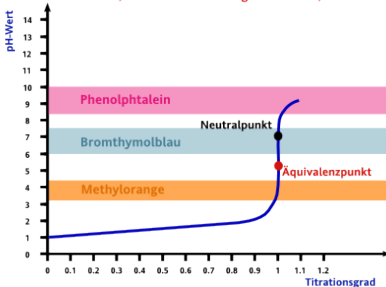
Titration of a 0.1M ammonium solution with a 0.1M hydrochloric acid solution
